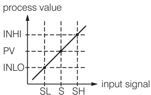
Figure 3.1 Conversion Curve for Linear Type Process Value
