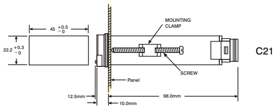
Figure 2.1 Mounting Dimensions
