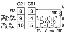
Figure 2.8 Sensor Input Wiring
