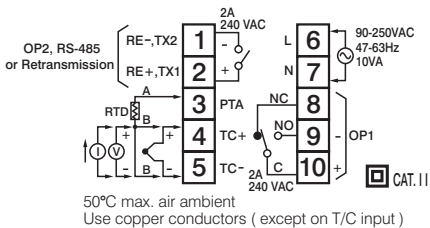
Figure 2.5 Rear Terminal Connection for C91
