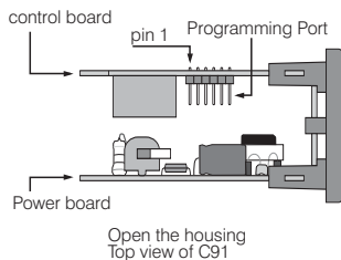
Figure 1.2 Programming Port Overview
